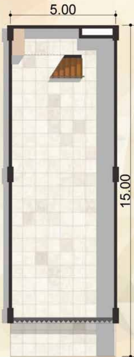
DENAH LANTAI 1
